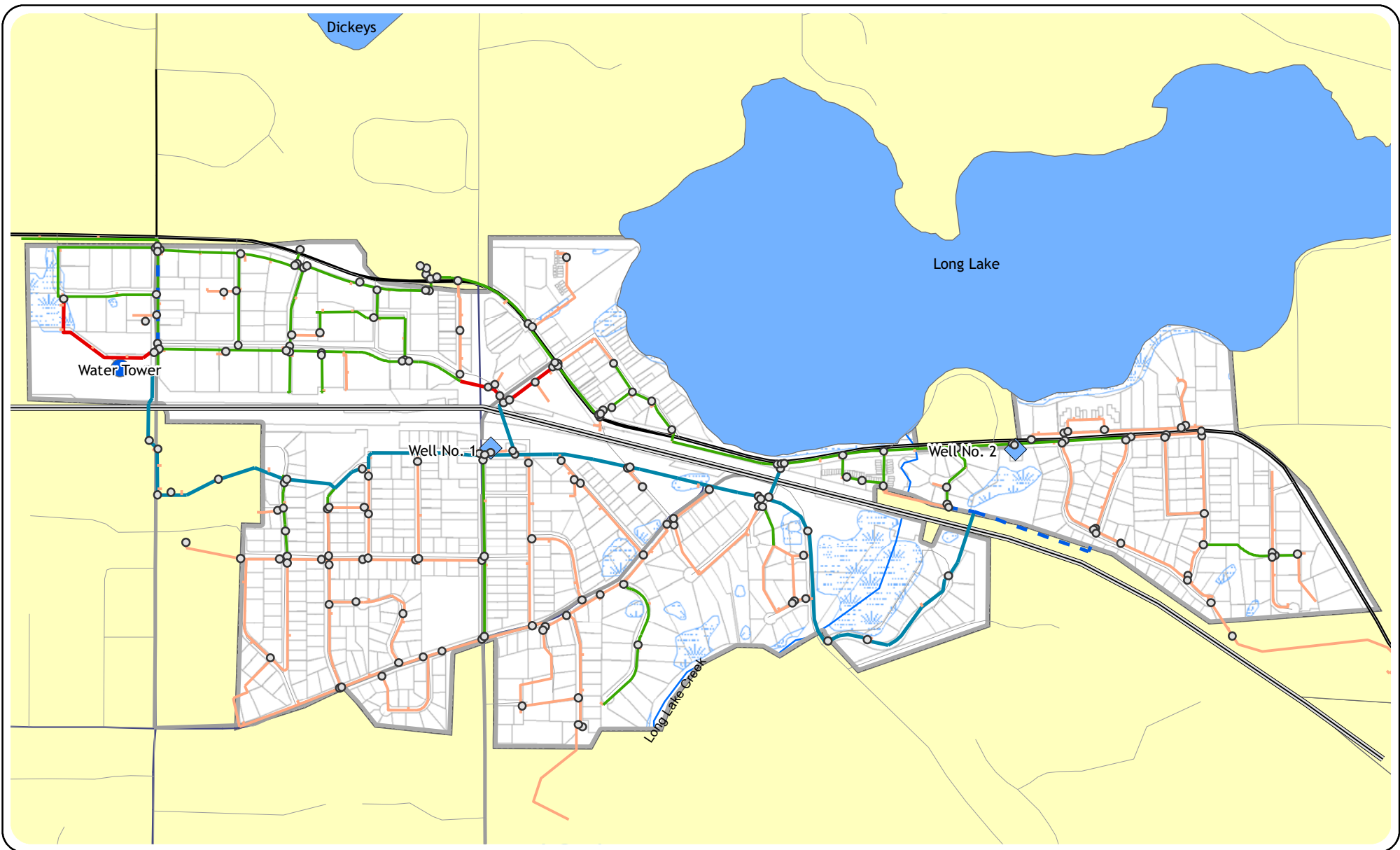
Figure 13 Water Distribution System
